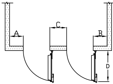
MULTIPLE DOORS PLAN VIEW
