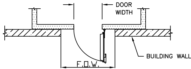
THRU-WALL INSTALLATION PLAN VIEW
