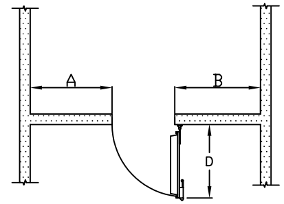
INTERIOR WALL DOORS PLAN VIEW
