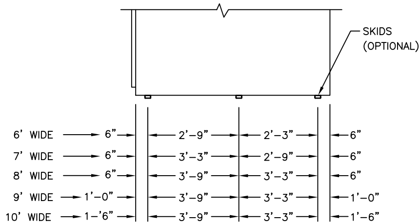
END ELEVATION 6' - 10' WIDE BUILDING
