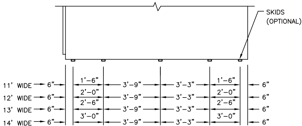
END ELEVATION 11' - 14' WIDE BUILDING
