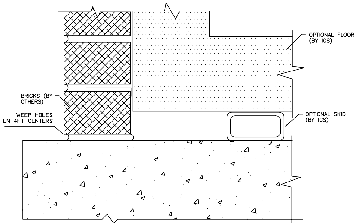
MASONRY BASE DETAIL
