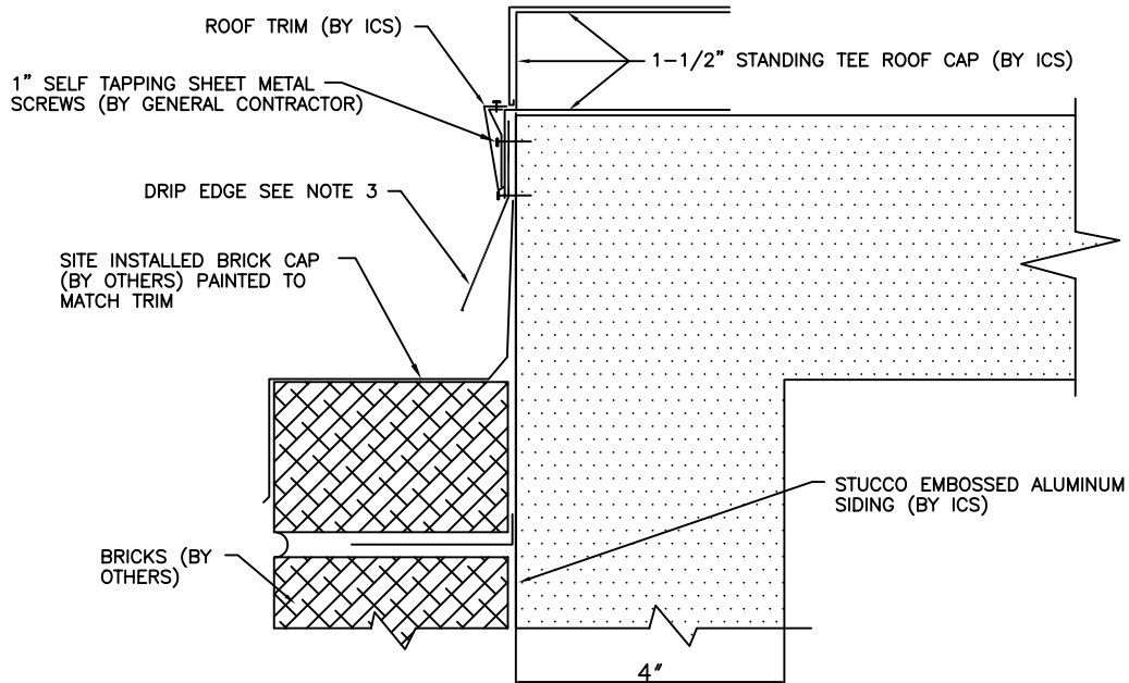
MASONRY CAP FLASHING DETAIL
