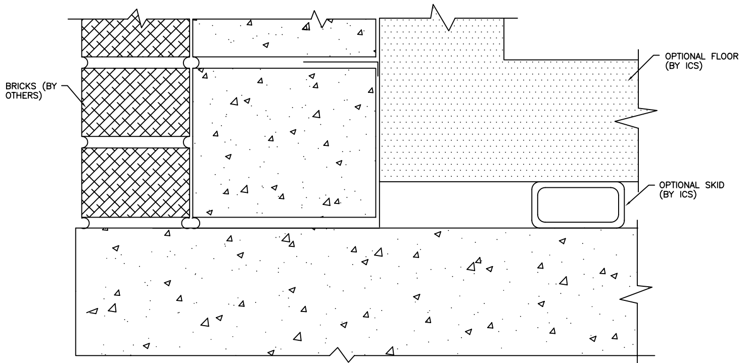
MASONRY BASE DETAIL
