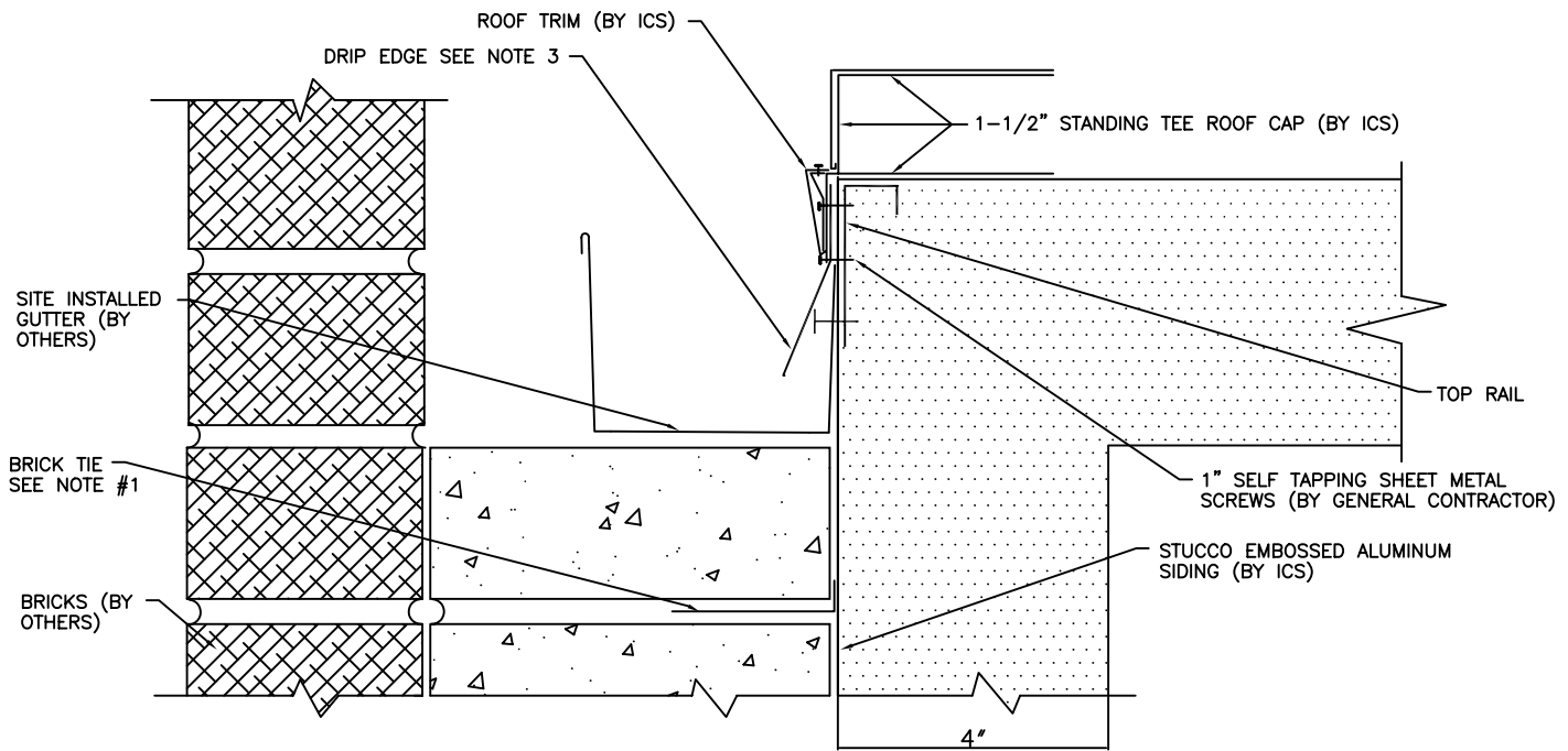
MASONRY CAP FLASHING DETAIL
