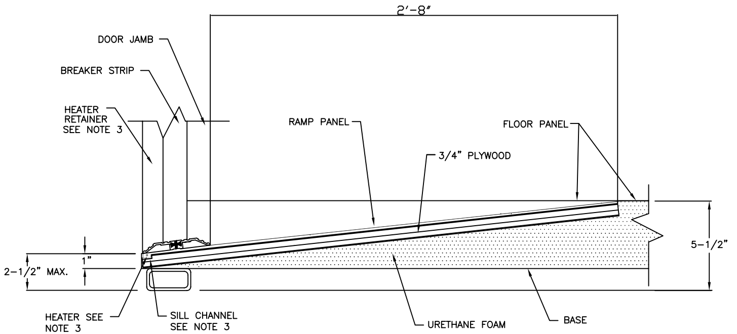
CROSS SECTION AT FLOOR RAMP
