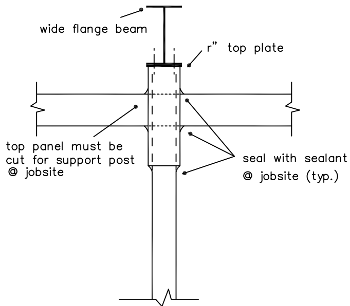
29C/D-BEAM SUPPORT COLUMN
