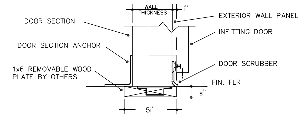
(A) TYPICAL DETAIL AT FLOOR
