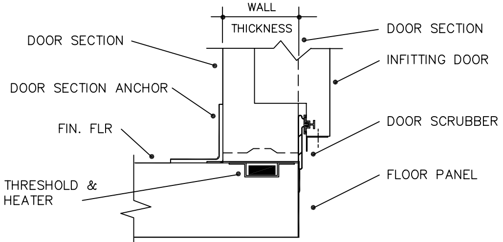
(A) TYPICAL DETAIL AT FOAM FLOOR SEE 4F.28 FOR NOTCH-OUT IN WOOD FLOOR
