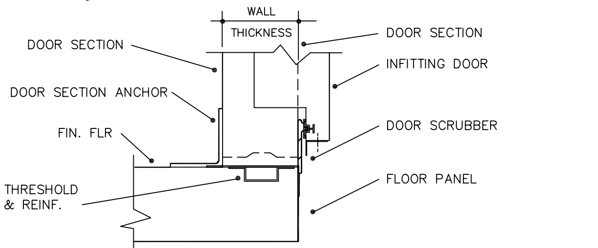
(A) TYPICAL DETAIL AT FOAM FLOOR SEE 4F.28 FOR NOTCH-OUT IN WOOD FLOOR
