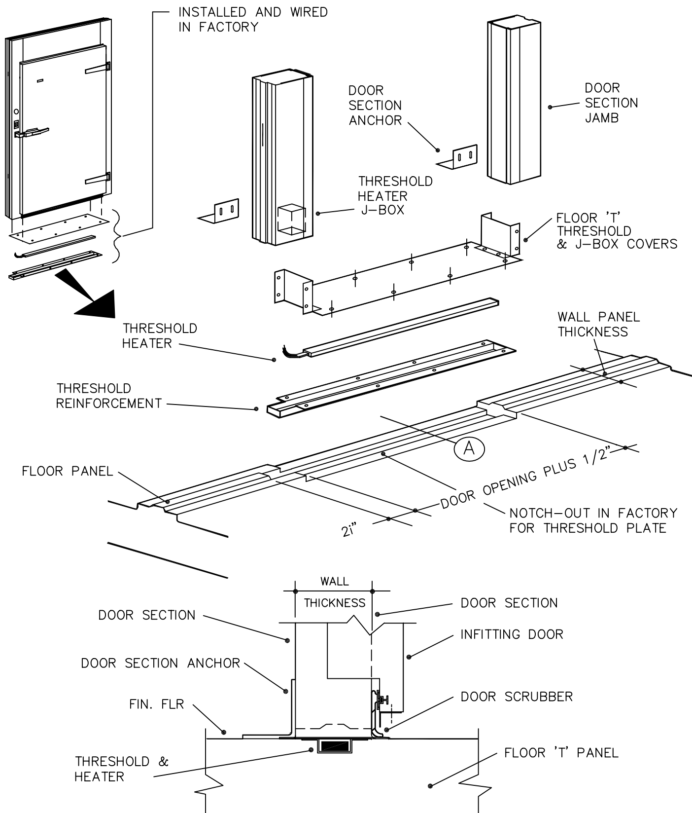
(A) TYPICAL DETAIL AT FOAM FLOOR SEE 4F.28 FOR NOTCH-OUT IN WOOD FLOOR
